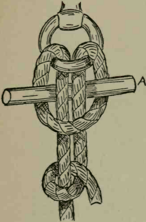
FIG. 30.—Lark's head with toggle (A).
